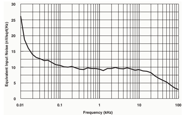
Figure 4. Equivalent input noise voltage vs. frequency
