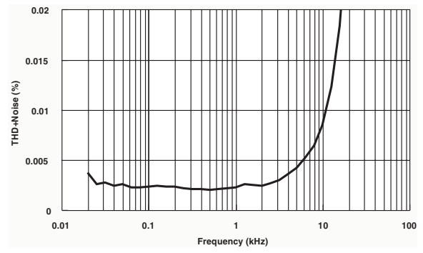
Figure 6. THD + noise vs. frequency
